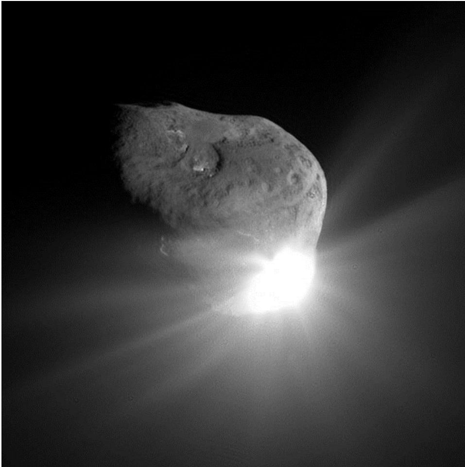
Figure 4. Comet Tempel 1 after being struck by the Deep Impact space probe in July 2005. Photo courtesy of NASA/Jet Propulsion Laboratory.
