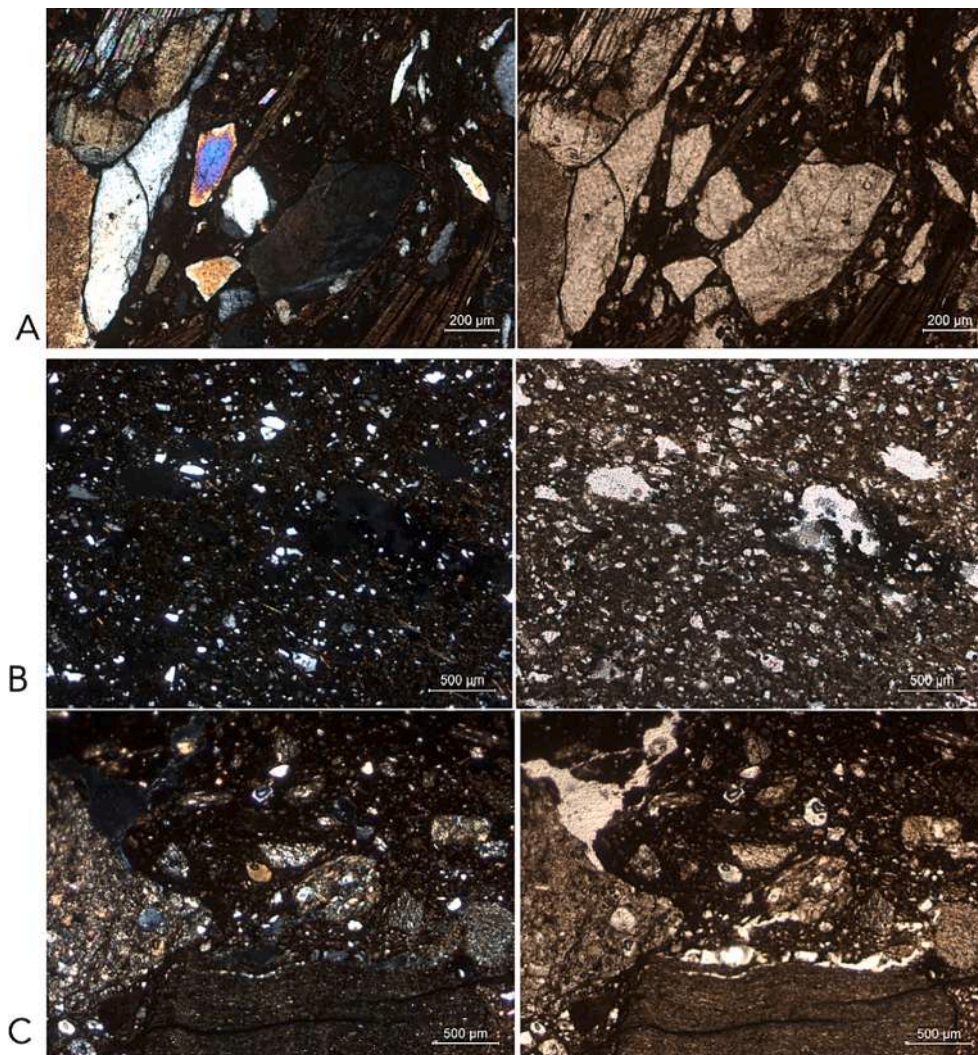
Fig. 7. Petrography microphotographies a) group A b) group B and c) group C.
