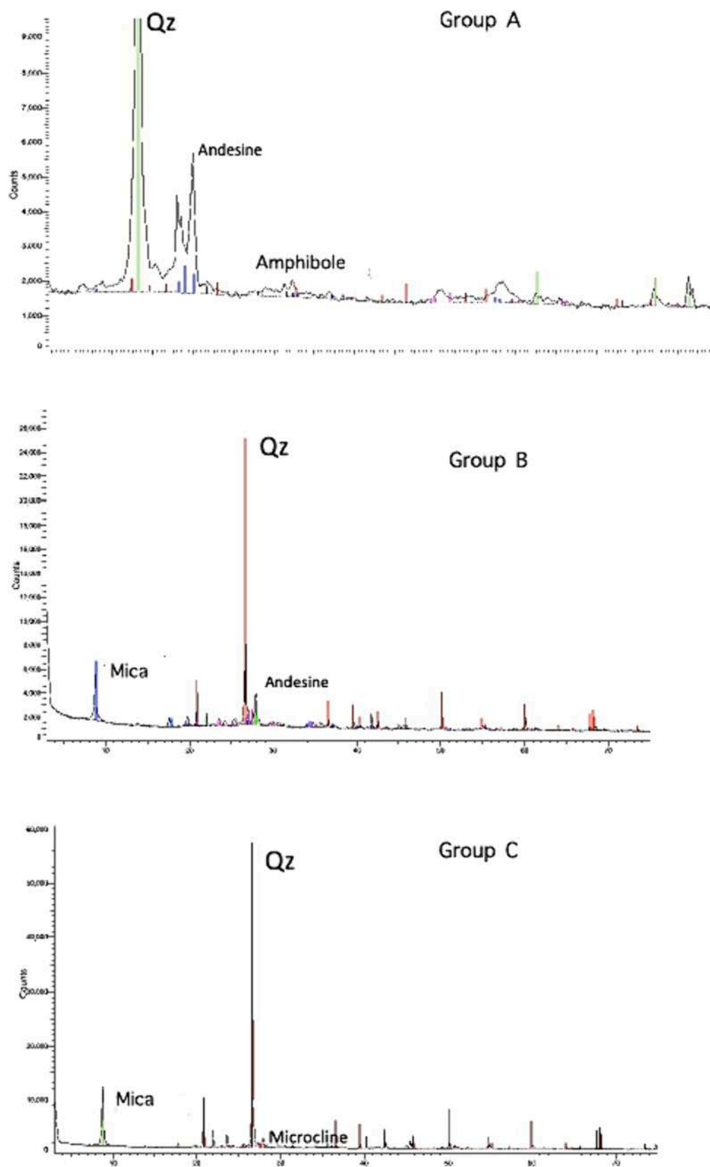
Fig. 5. XRD diffractograms from each petrographic group.
