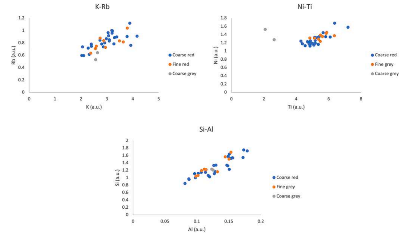
Fig. 4. Pxrfl biplots. samples cluster in a discrete and homogenous group, except for coarse grey group samples that are slightly deployed in ti.
