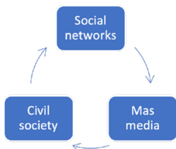
Figure 3. Disinformation strategy
